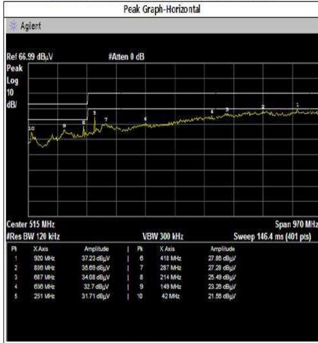
Radiated Emission Data Graph (30 MHz ~ 1GHz) 동작_2024.09.19
