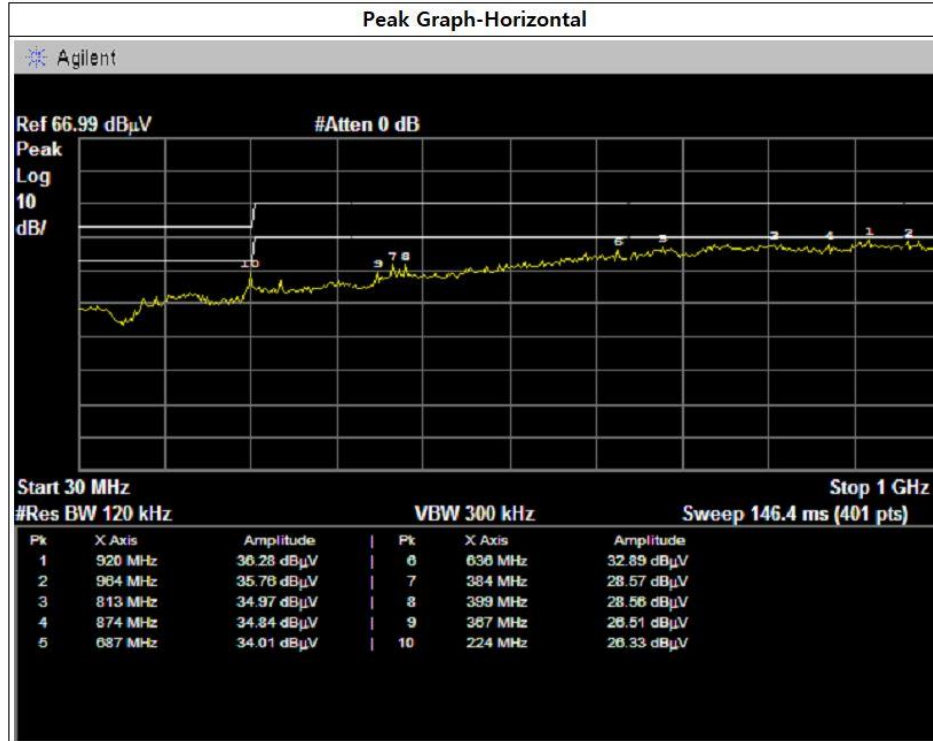
Radiated Emission Data Graph ( 30 MHz ~ 1 GHz ) 동작 (2024.08.24)
