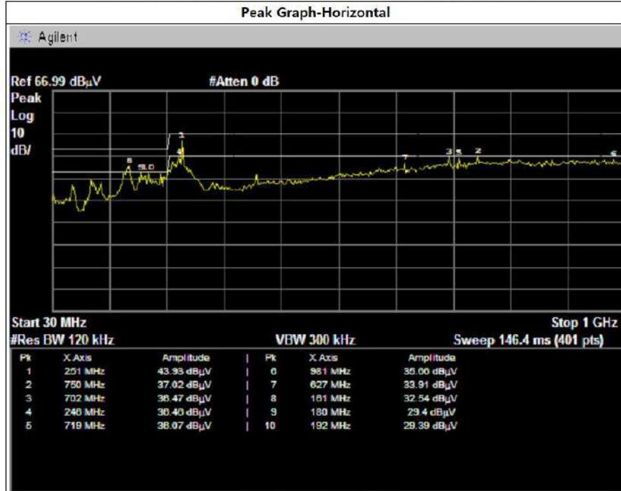
Radiated Emission Data Graph ( 30 MHz ~ 1 GHz ) 동작 2024.08.23
