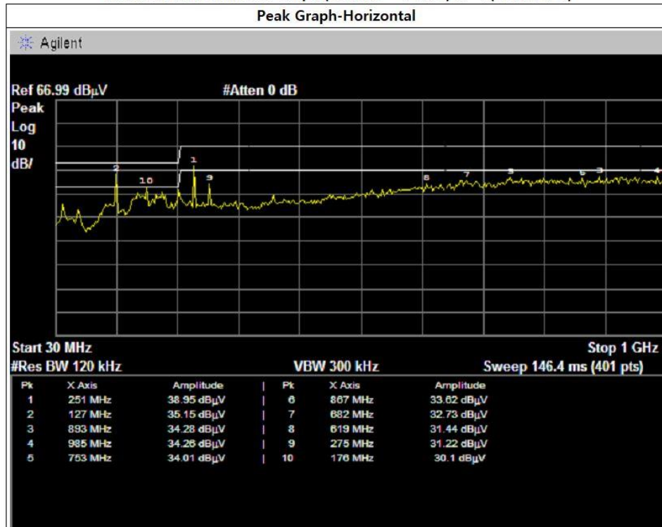
Radiated Emission Data Graph ( 30 MHz ~ 1 GHz ) 동작 (2024.08.24)
