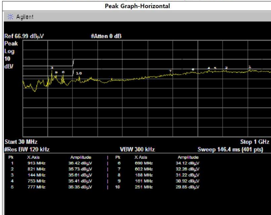
Radiated Emission Data Graph ( 30 MHz ~ 1 GHz ) 동작 2024.08.23
