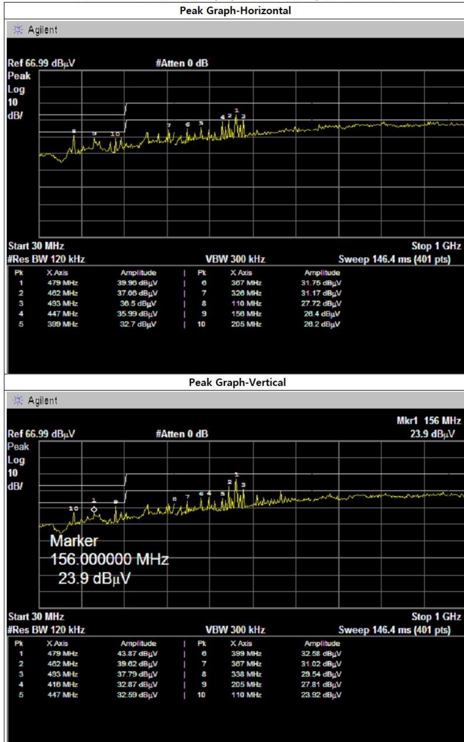
Radiated Emission Data Graph ( 30 MHz ~ 1 GHz ) 동작 2024.08.21
