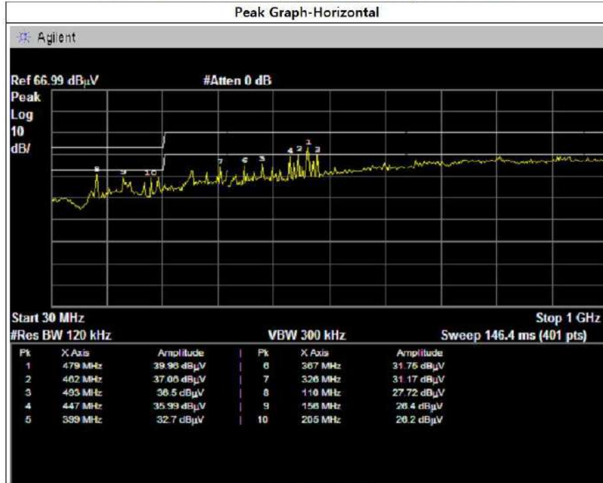
Radiated Emission Data Graph ( 30 MHz ~ 1 GHz ) 동작 2024.08.21
