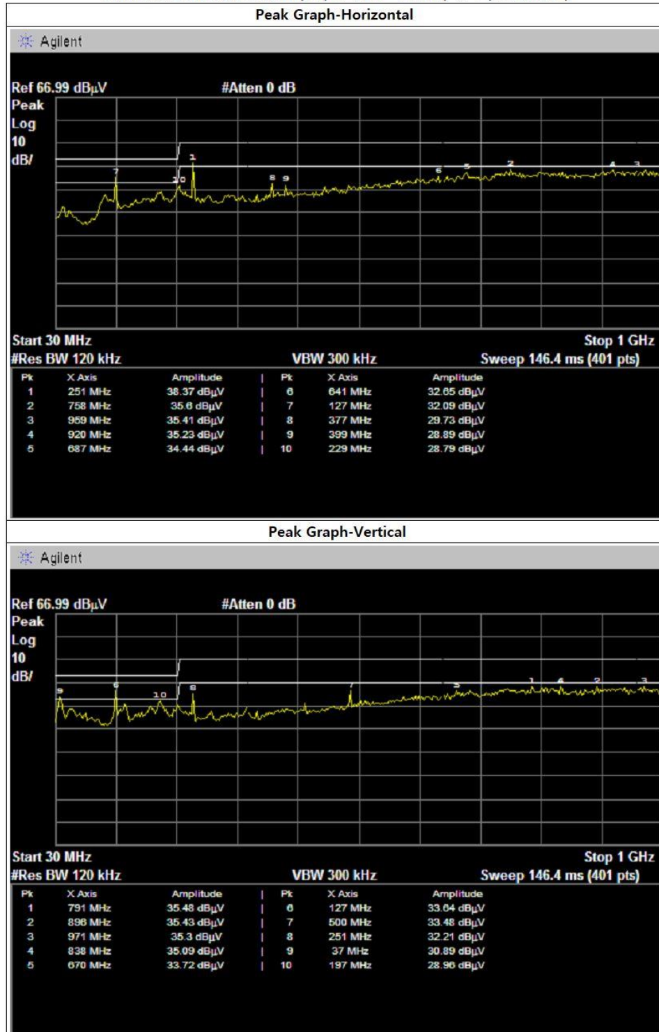
Radiated Emission Data Graph ( 30 MHz ~ 1 GHz ) 동작 (2024.08.24)
