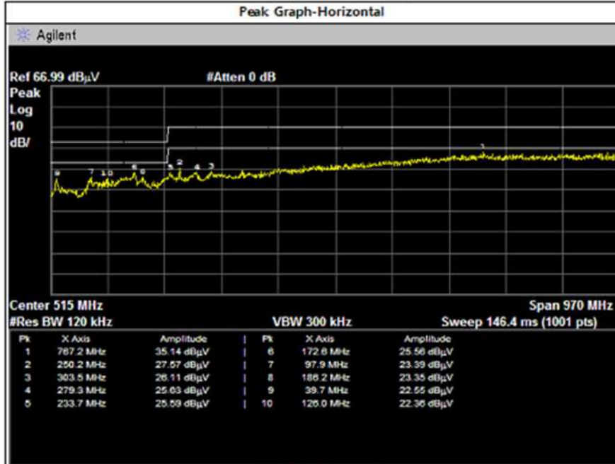
Radiated Emission Data Graph ( 30 MHz ~ 1 GHz ) DC 60 V 2025.09.22
